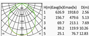
MTC 2835 LED 80W 5044lm Opal PC 113° Class I, IP65
