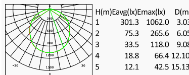
MTC 2835 LED 45W 3370lm Opal PC 113° Class I, IP65
