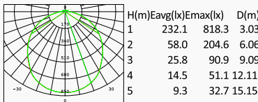
MTC 2835 LED 30W 2596lm Opal PC 113° Class I, IP65
