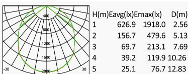
MTC 2835 LED 80W 5044lm Opal PC 113° Class I, IP65
