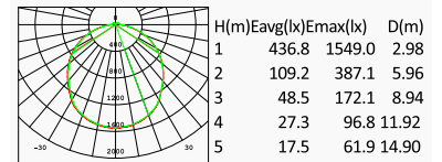
MTC 2835 LED 60W 4888lm Opal PC 113° Class I, IP65
