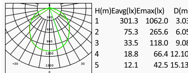
MTC 2835 LED 45W 3370lm Opal PC 113° Class I, IP65
