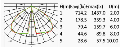
CREE LED 45W 3869lm Clear glass Class I, IP65
