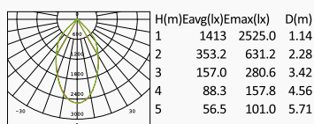
CREE LED 30W 2632lm Clear glass Class I, IP65
